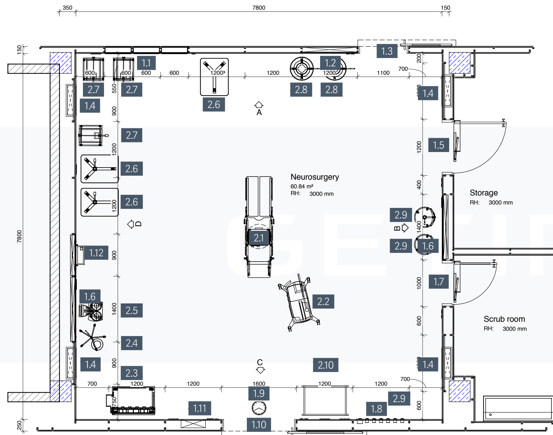
Groundplan
