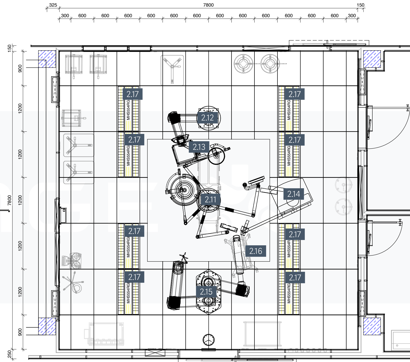
Ceilingplan
