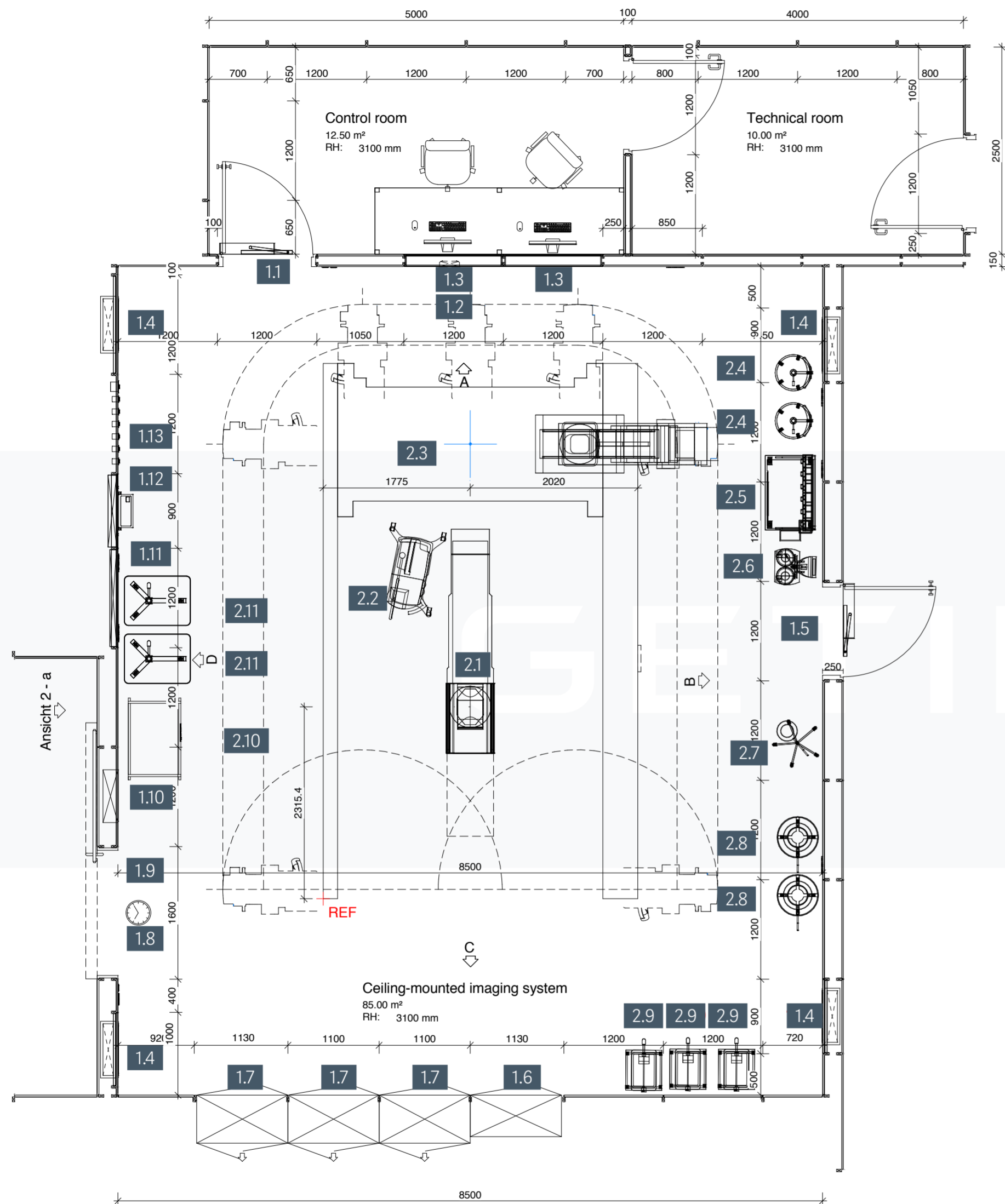
Groundplan
