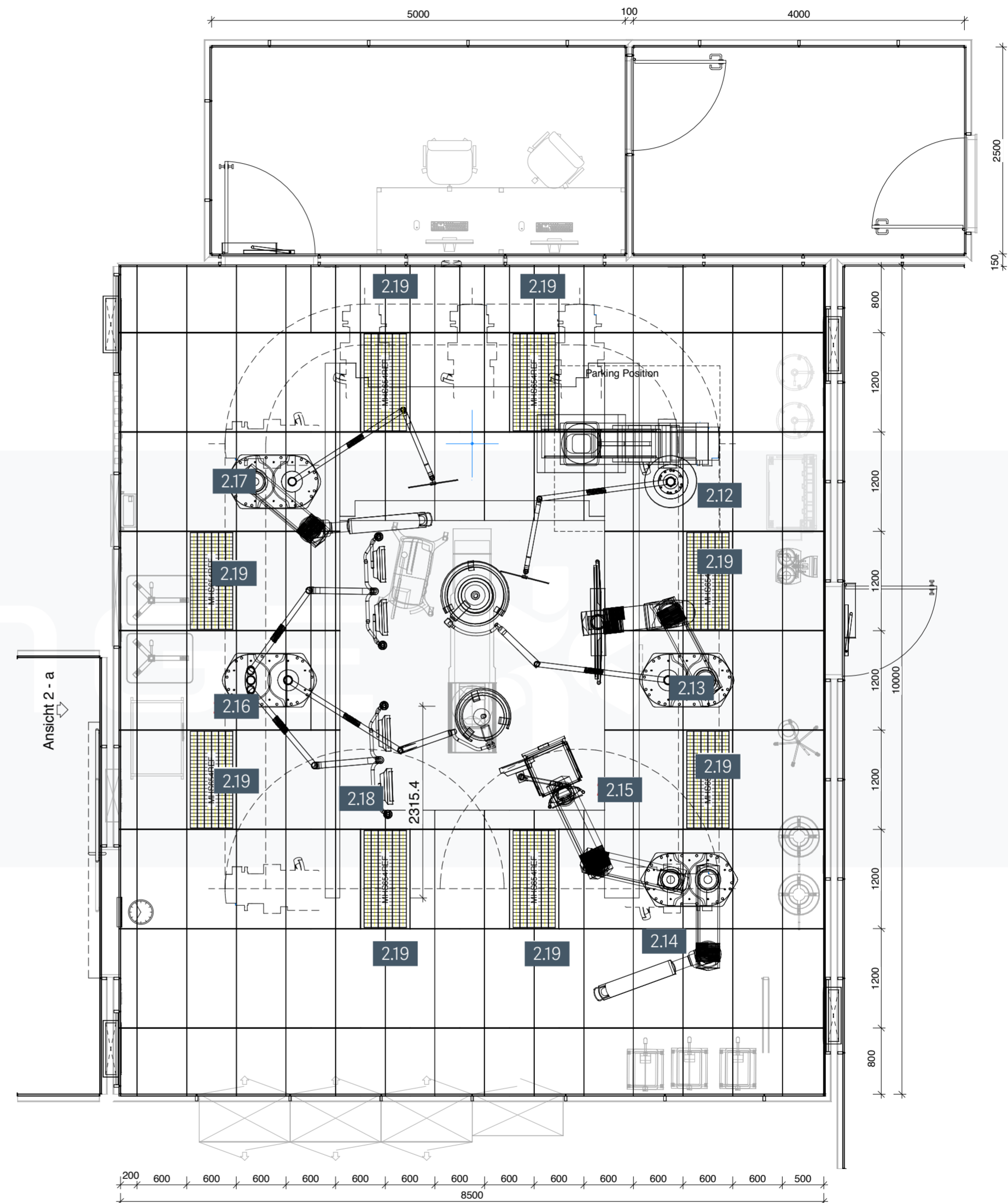
Ceilingplan
